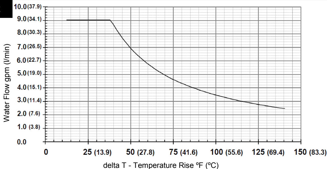
FLOW TABLE
